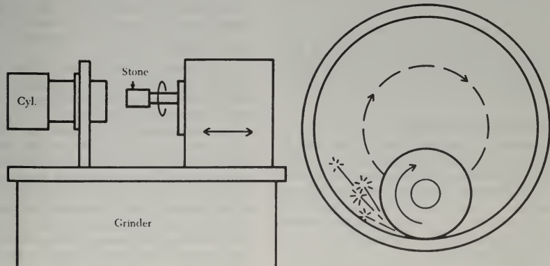
FIGURE 10-20. Cylinder bore grinding.
